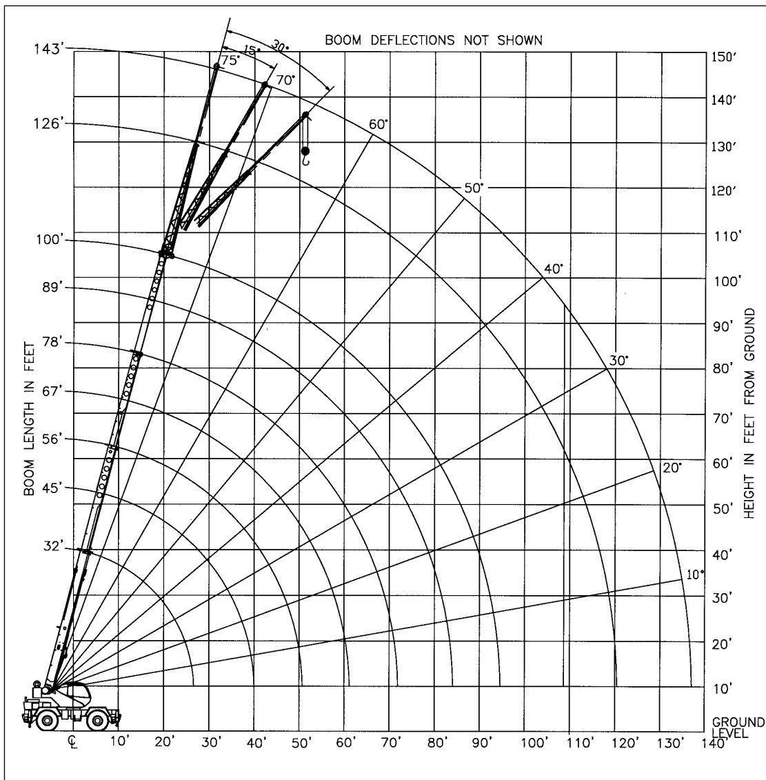
Range Diagram (32' - 100' boom)
