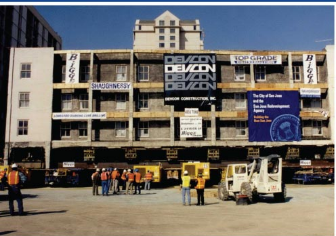
Montgomery Hotel 4800 ton move – San Jose, CA
